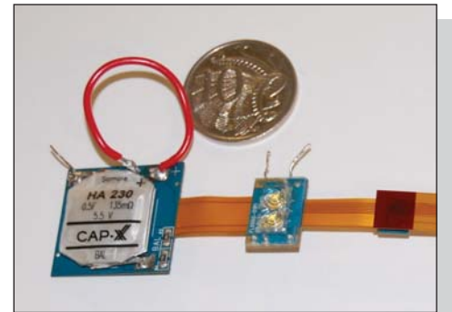
Figure 3a. Supercapacitor LED flash module with CAP-XX HA230 supercapacitor, AnalogicTech AAT1282 flash driver on the reverse side and Seoul Semiconductor LEDs.
