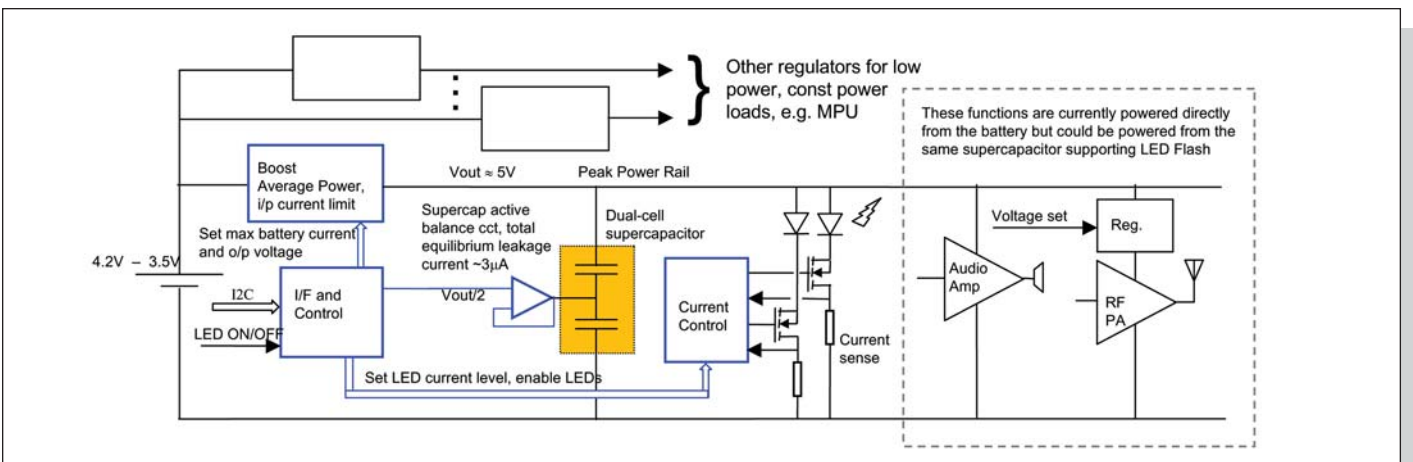
Figure 2. BriteFlash power architecture for high-power LED flash using a supercapacitor
