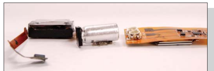
Figure 3b. Supercapacitor LED flash module with the CAP-XX HA230 on the underside, ON Semiconductor's NCP5680 flash driver and Lumileds LEDs. Also pictured is the Nokia N82 xenon solution with large cylindrical electrolytic.
